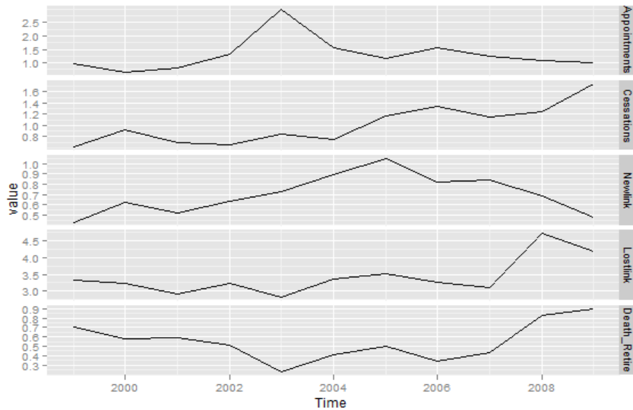
Figure 3: Network Dynamics
